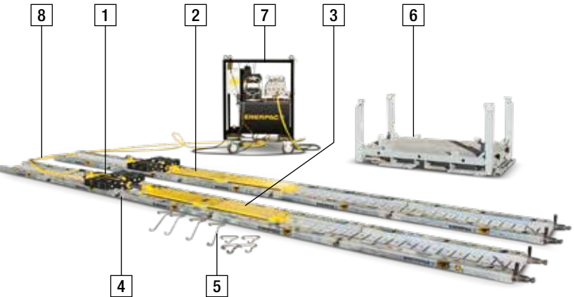
LH-Series, Low-Height Skidding System (dimensions in inches)
