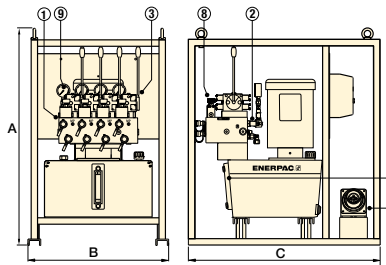
SFP-Series with 10 gallons reservoir (shown with 4 split-flow outlets)
