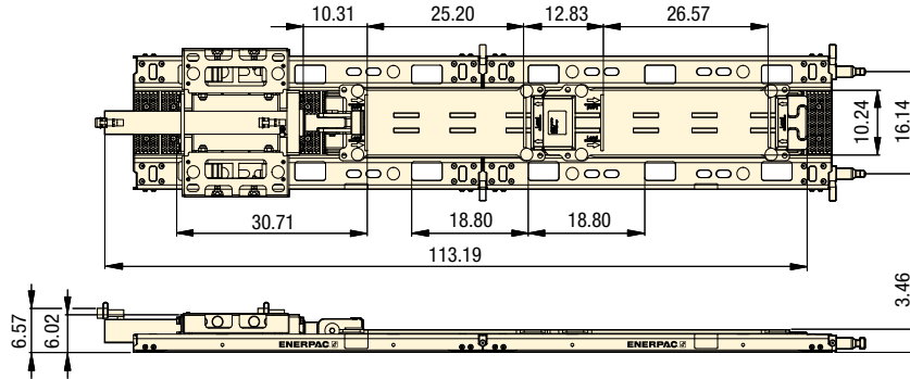
LH-Series, Low-Height Skidding System (dimensions in inches)
