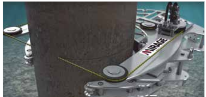
▼ Subsea pile cutting.
