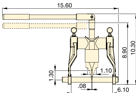
Tool retracted and advanced using large (ø 0.80 inch) spreading bar
