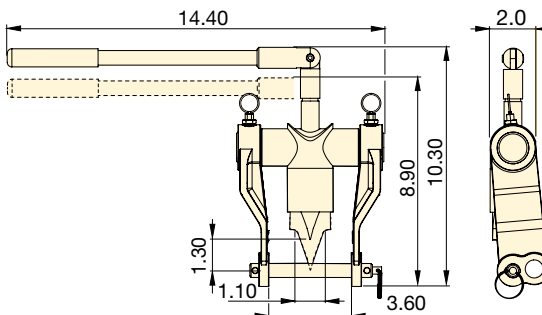
Tool retracted and advanced using small (ø 0.60 inch) spreading bar
