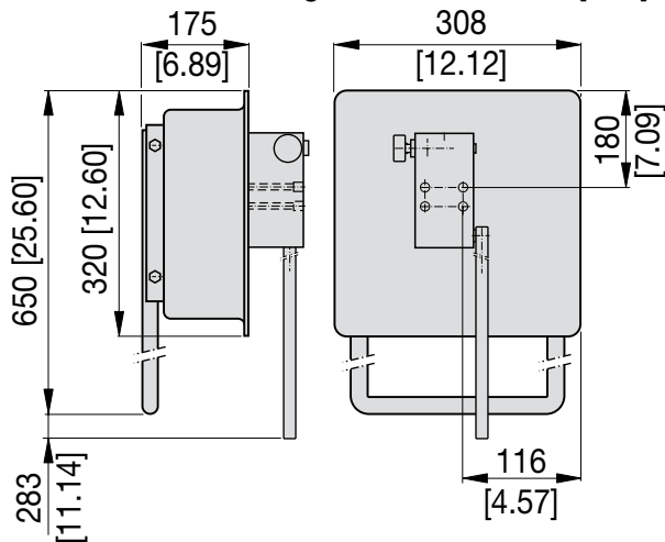
MP-10T Tank mounting dimensions in mm [inch]
