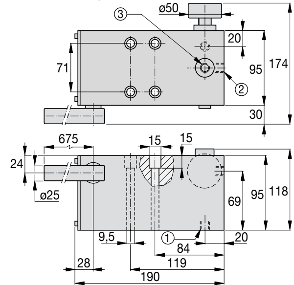
MP-Series Pump dimensions in millimeters
