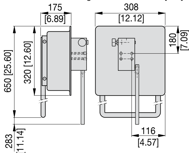
MP-10T Tankmonteringsdimensioner i mm [tum]
