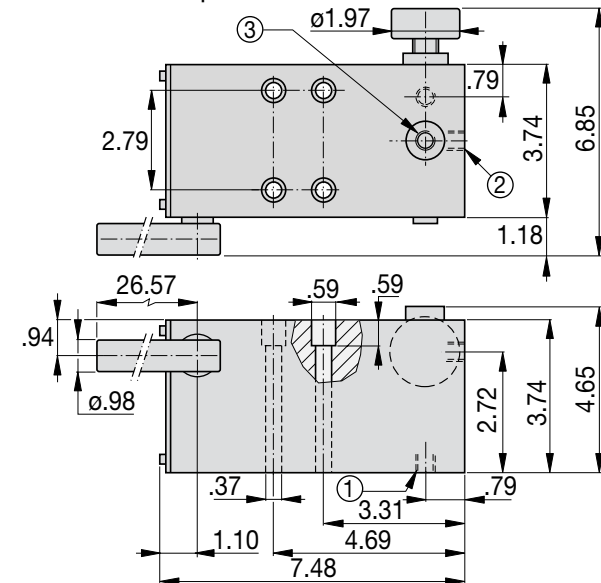
MP-Series Pump dimensions in inches
