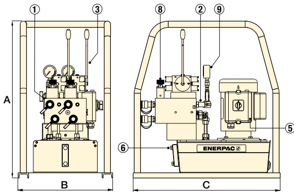
◀ SFP-Series with 2.5 gallons reservoir (shown with 2 split-flow outlets)
