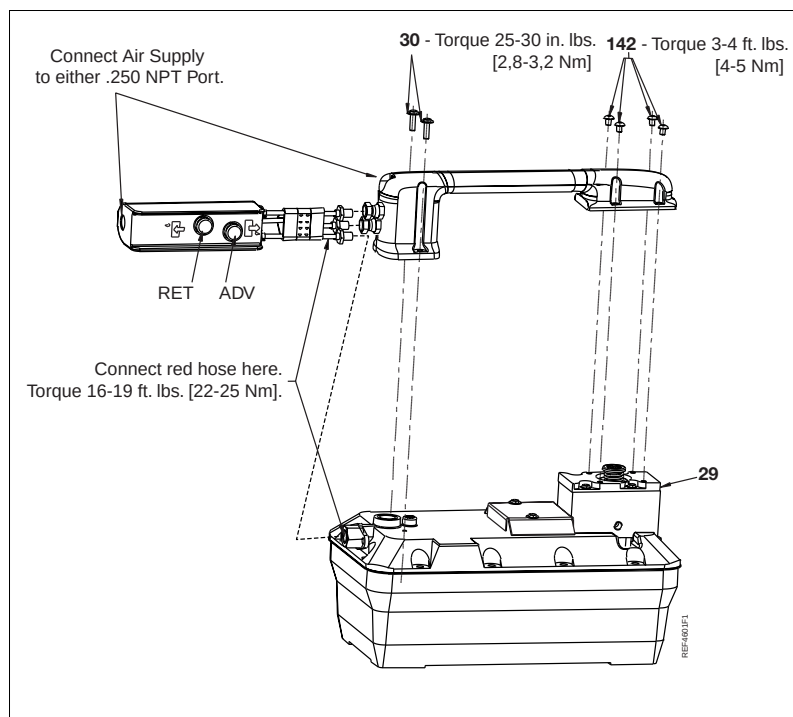
Figure 2a, Remote Pendant Turbo Pump Assembly
