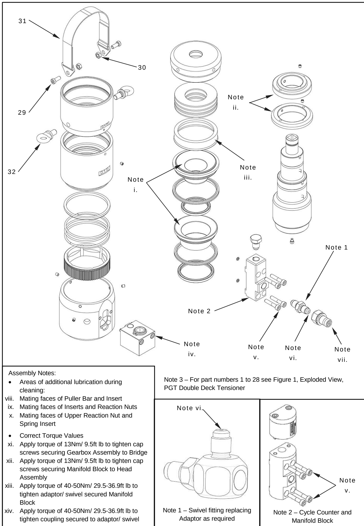
Figure 2, Exploded View, PGT Double Deck Tensioner with Lift Supports
