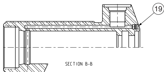
Figure 1, Threaded Body Mounting Style
