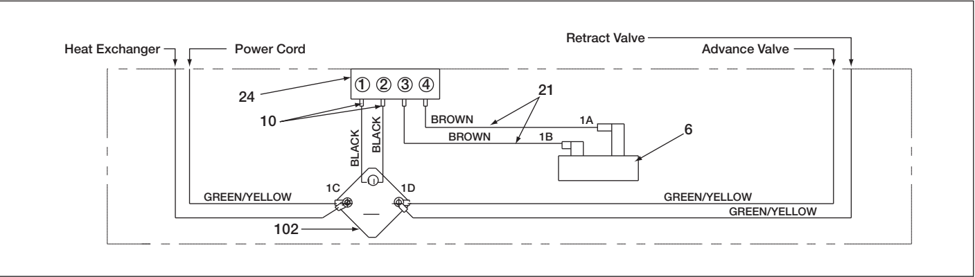
Figure 8, Wiring Diagram
