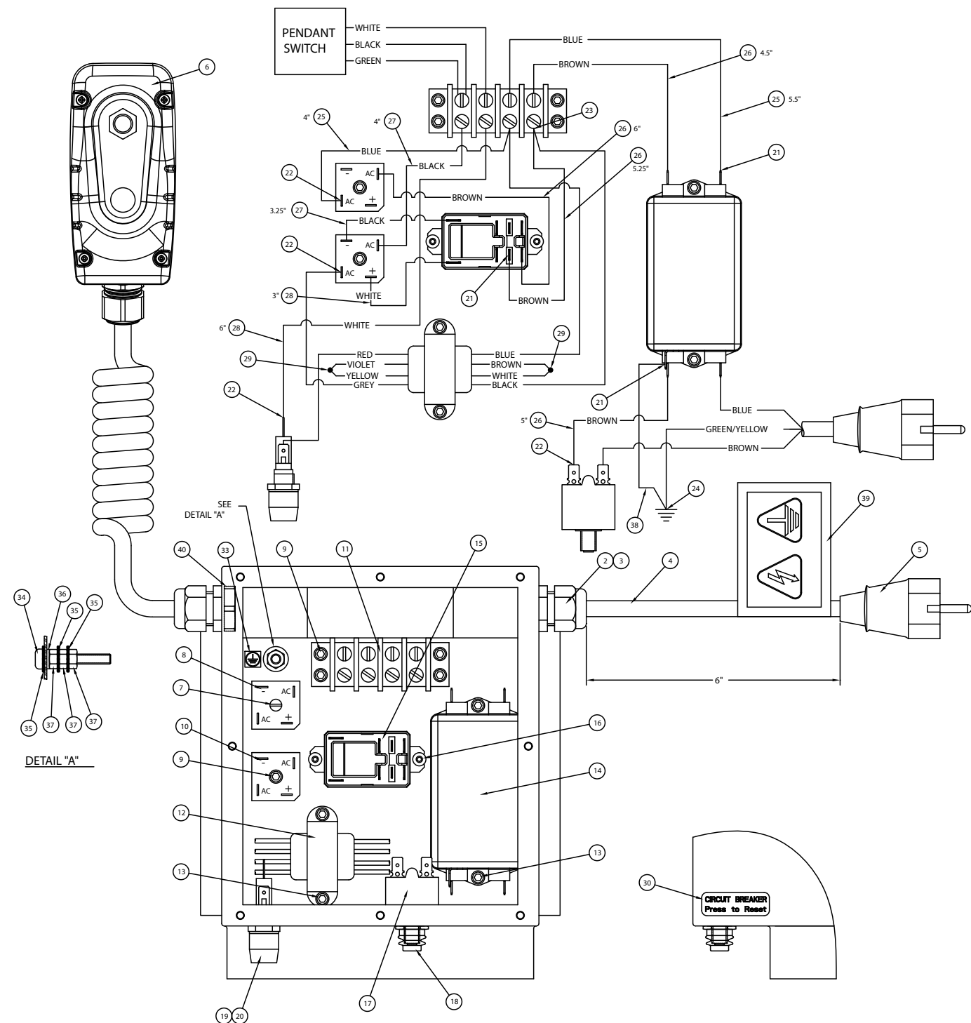
Figure 18A - DS1173900SR Shroud Electrical Assembly (230 V European)
