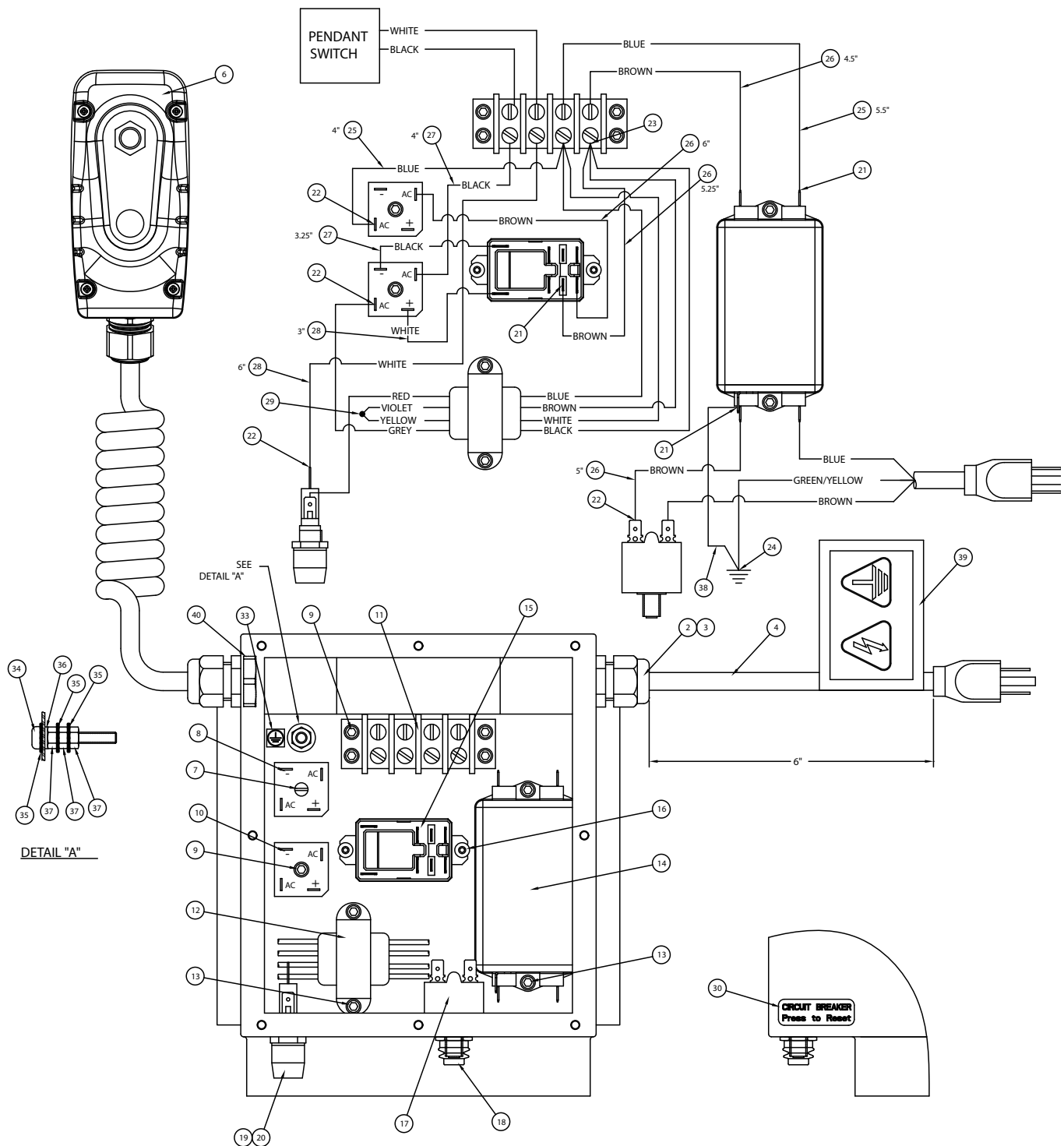
Figure 16A - DS1061900SR Shroud Electrical Assembly (115 V)
