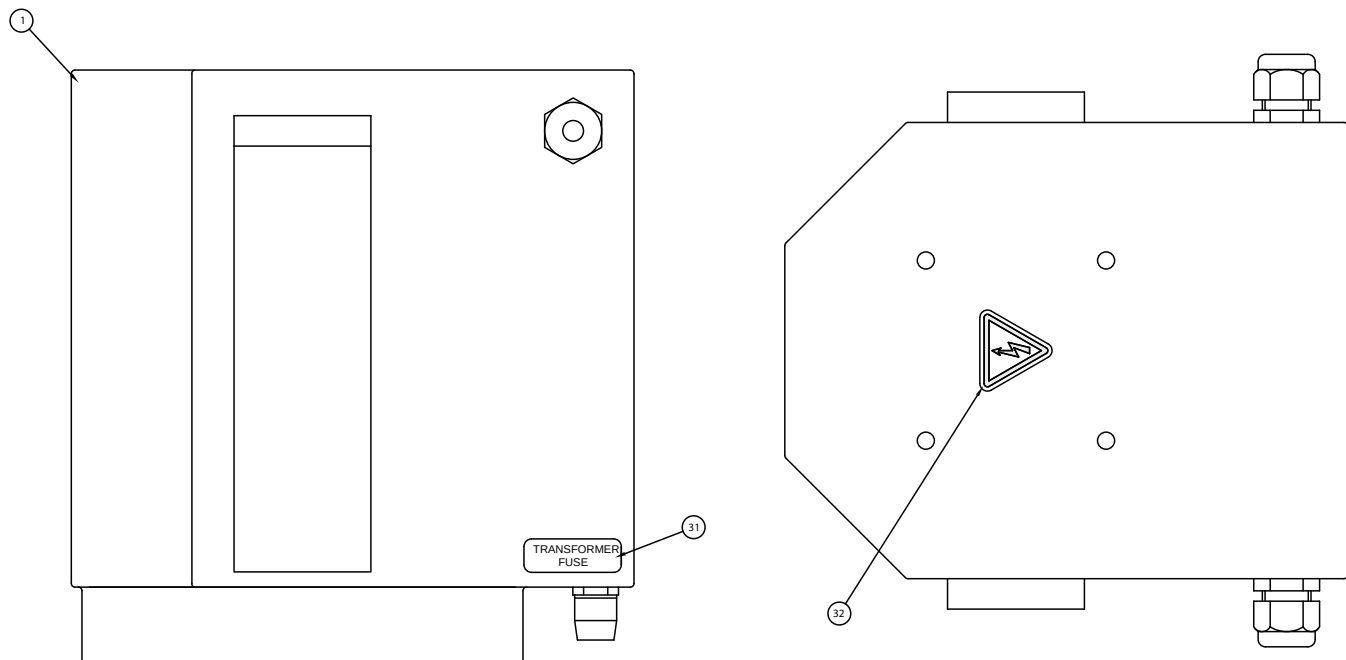
Figure 16B - DS1061900SR Shroud Electrical Assembly (115 V)
