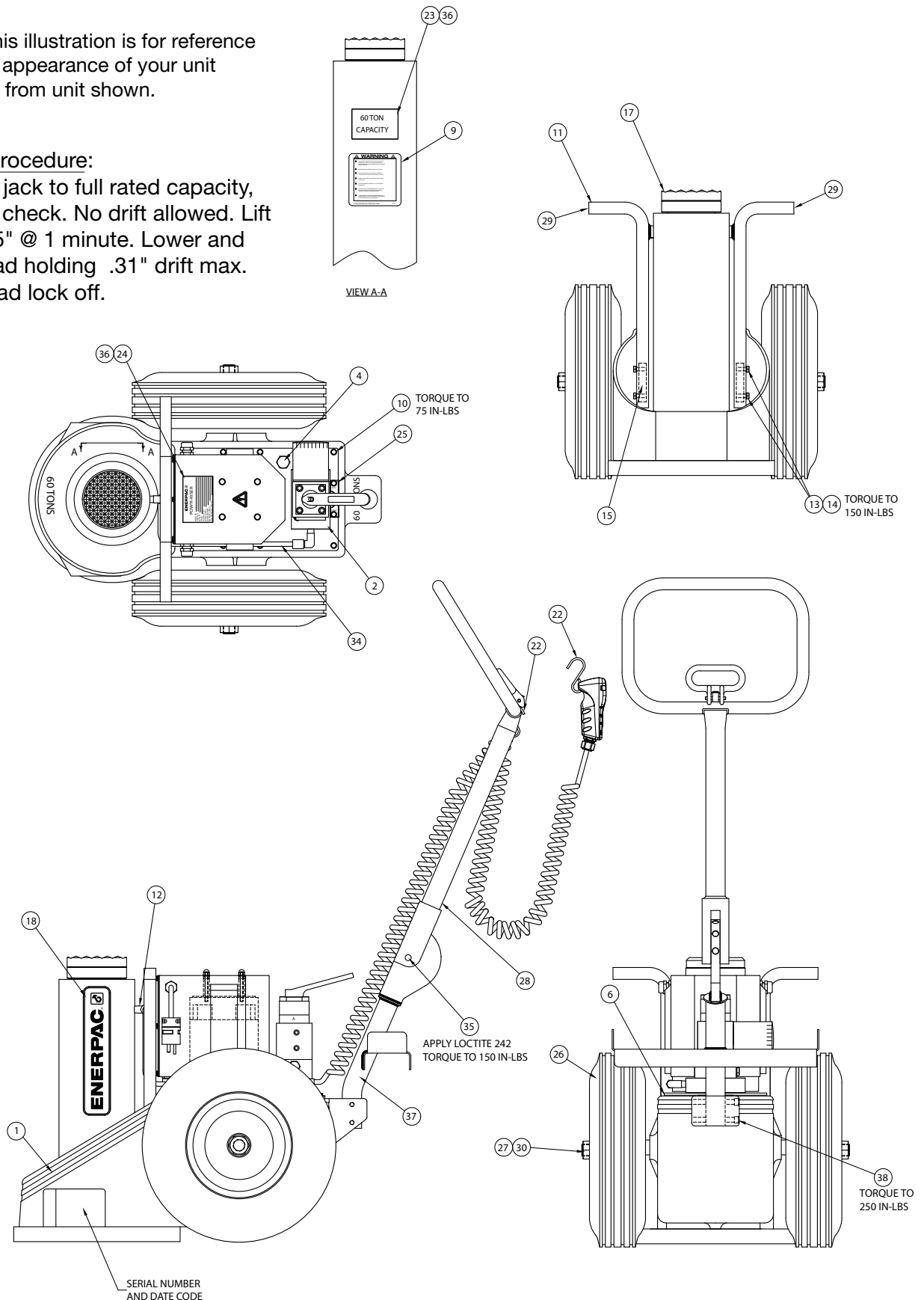
Figure 1 - Main Assembly
