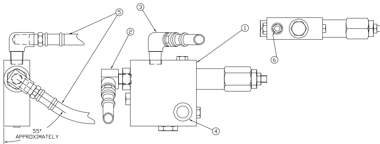
Figure 11 - 42353SR OC Valve Subassembly
