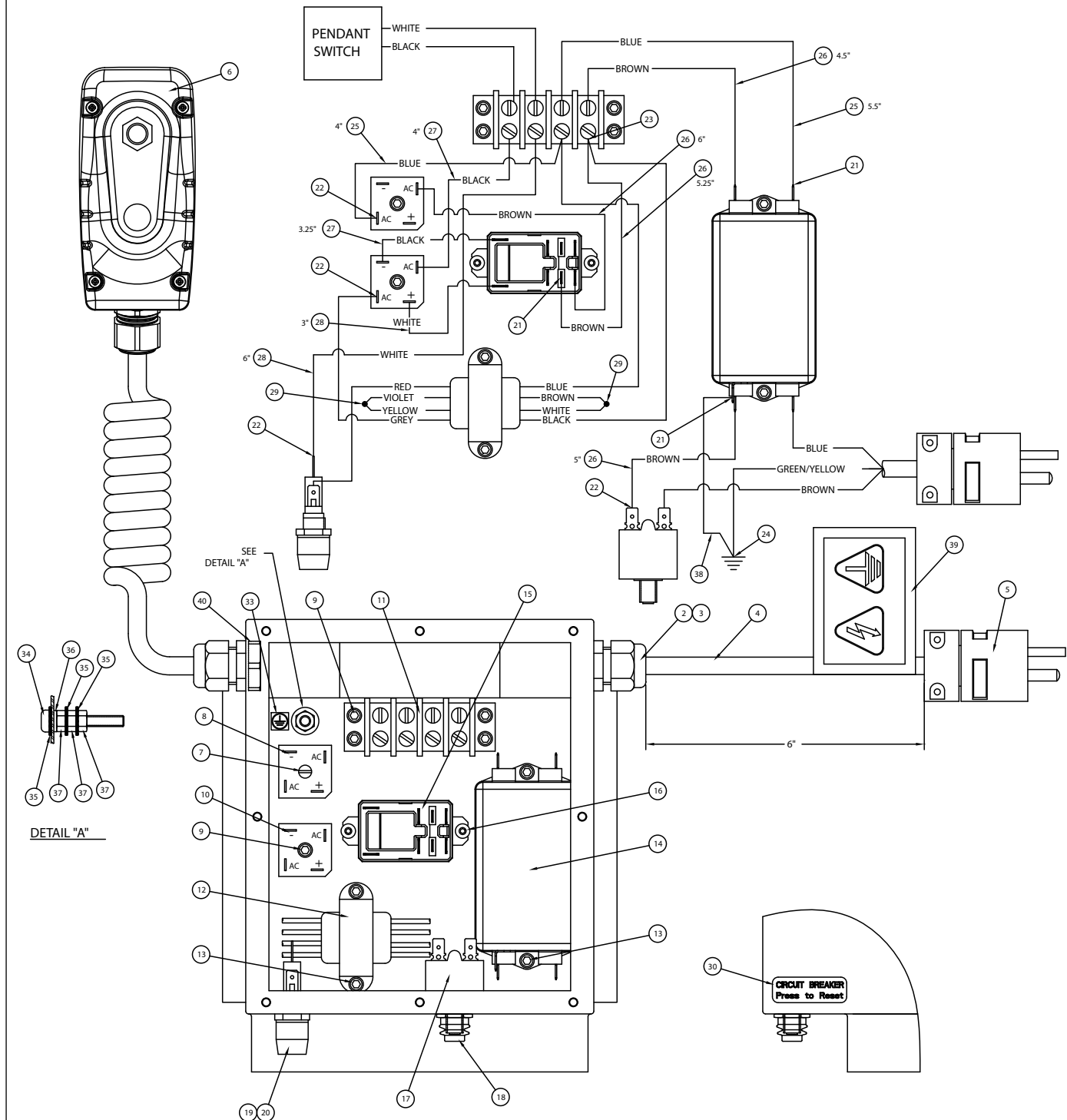
Figure 17A - DS1062900SR Shroud Electrical Assembly (230 V)
