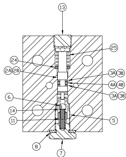
Figure 14 - 42480SR Locking Valve Subassembly (with relief)
