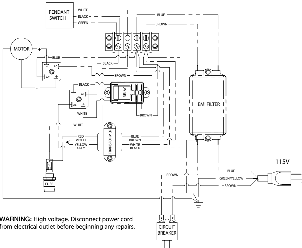
Figure 19 - 115 Volt Wiring Diagram
