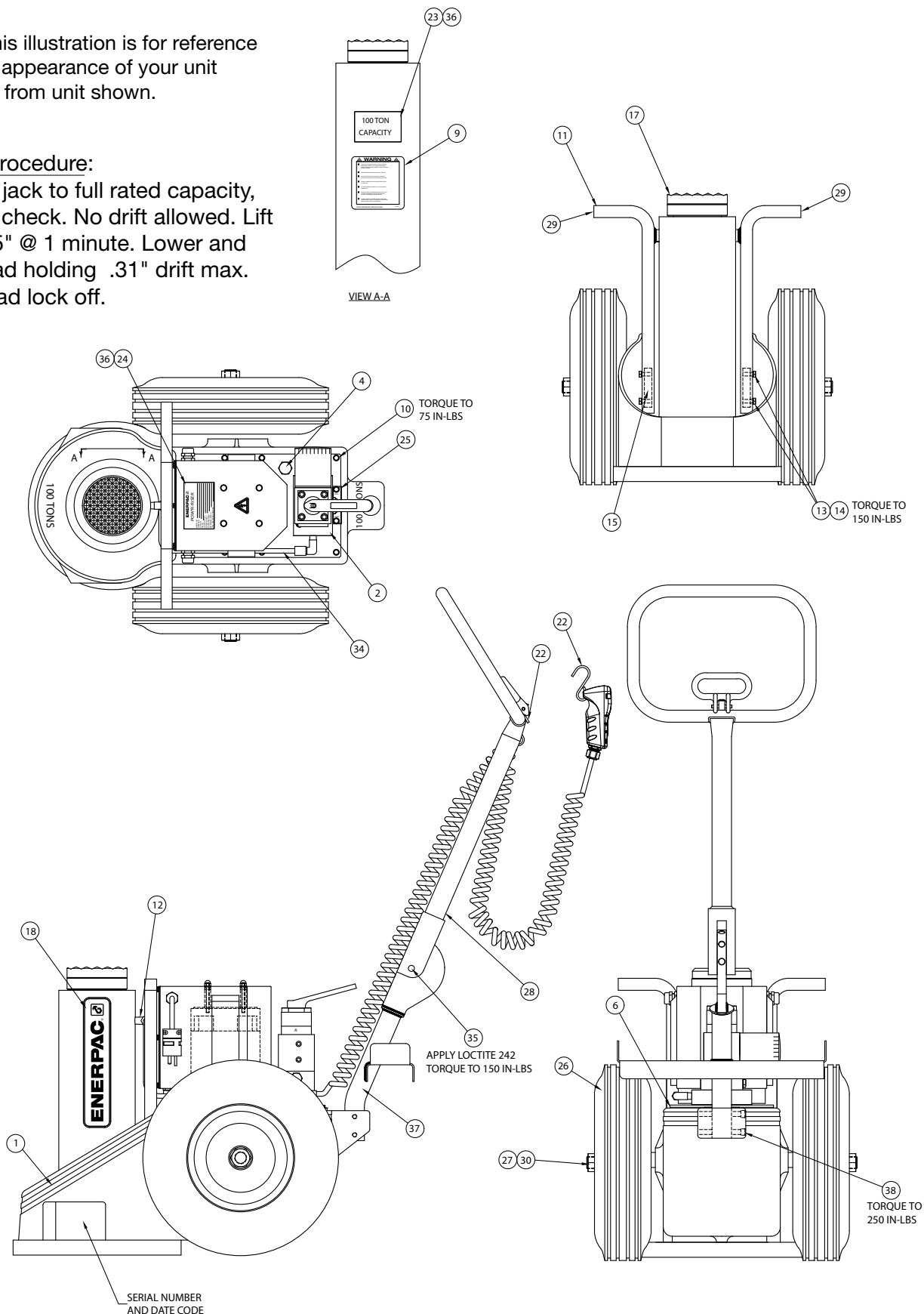
Figure 1 - Main Assembly
