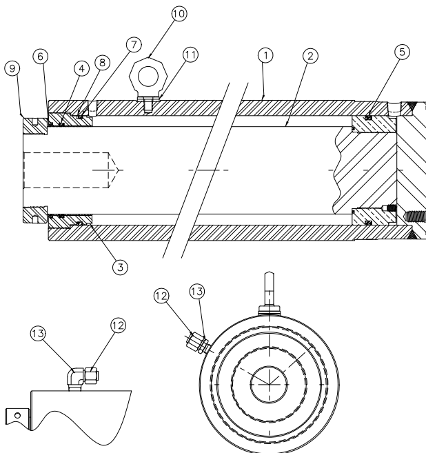
Figure 12 - S42050SR, 41926SR Cylinder Asm.
