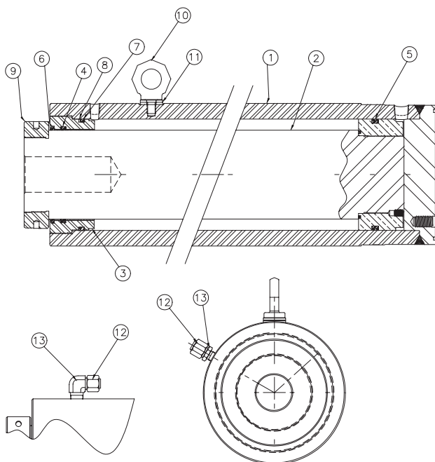
Figure 12 - S42050SR, 41926SR Cylinder Asm.
