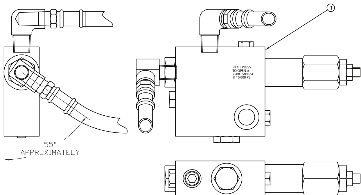
Figure 11 - 42353SR Over-Center Valve Subassembly
