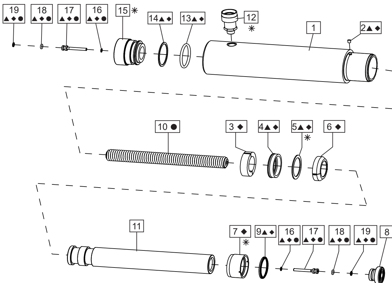
Fig. 1, Cylinder Assembly
