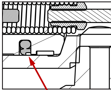
❖ Piston seal orientation
