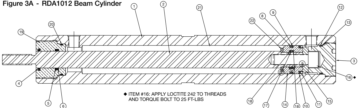
Figure 3A - RDA1012 Beam Cylinder
