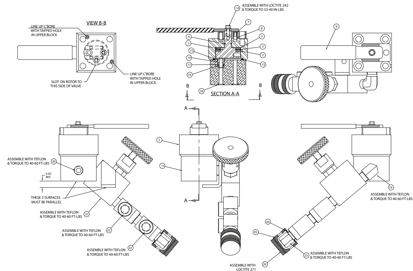
Figure 5 - 46066SR Control Valve Subassembly
