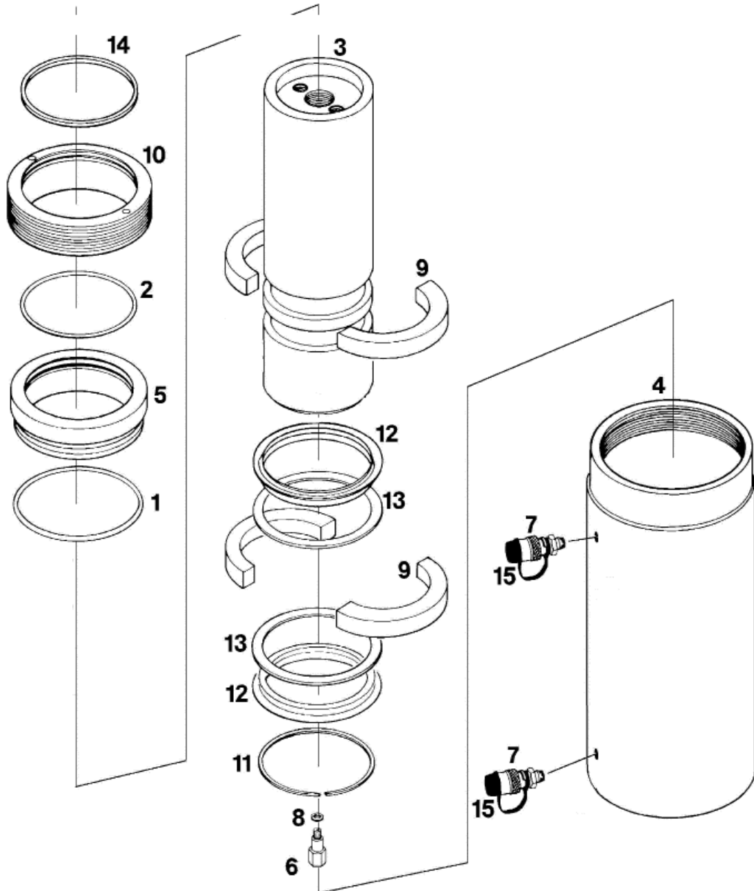
75 Ton 4.63" Stroke Double-Acting Hydraulic Cylinder
