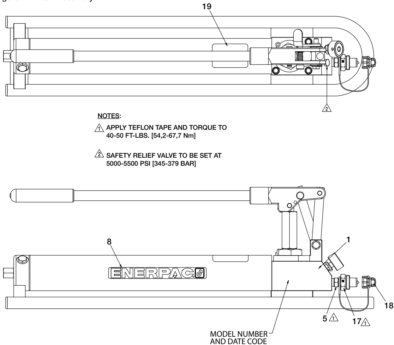
Figure 1 - Main Assembly
