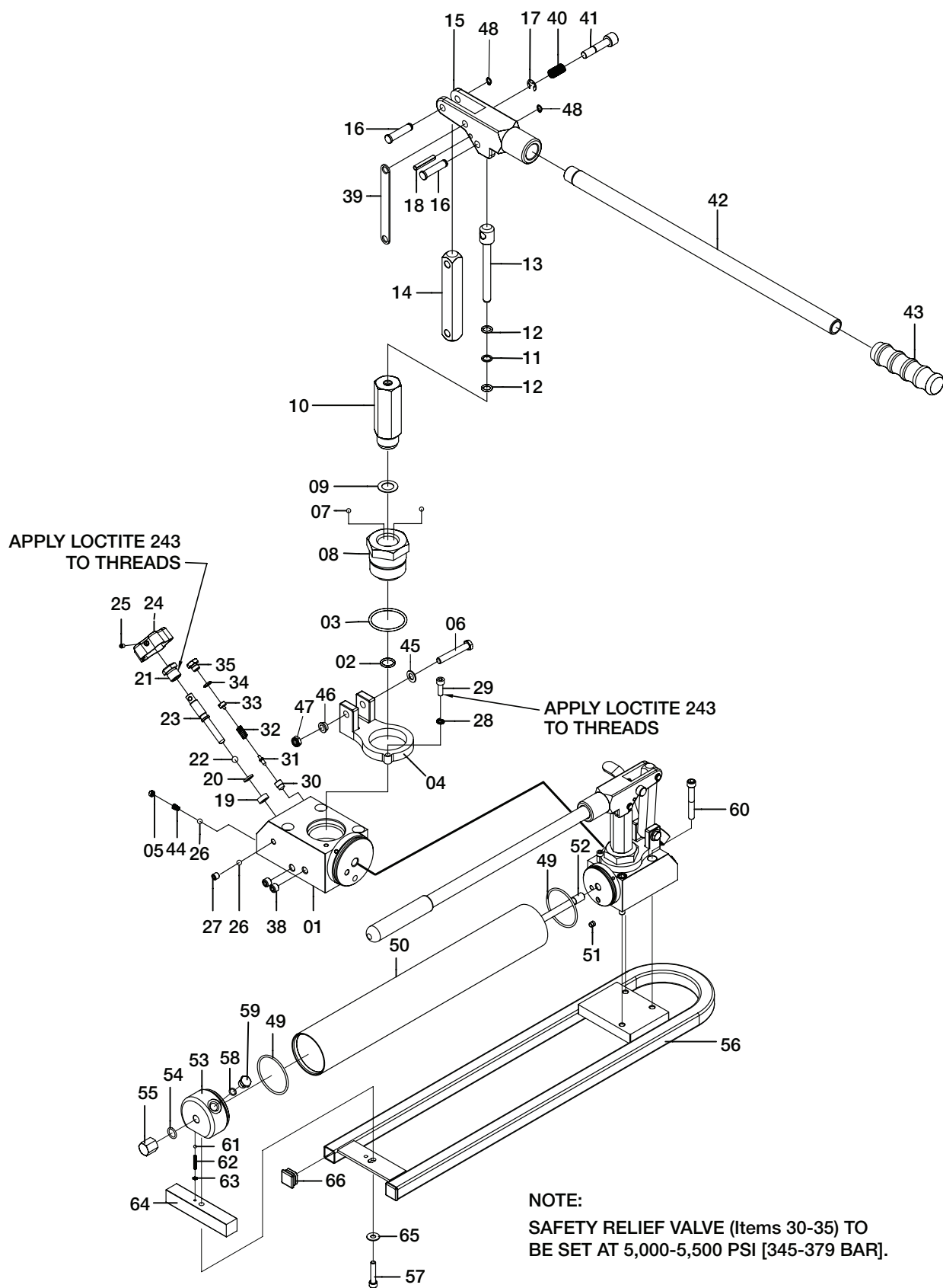
Figure 2 - Pump Assembly
