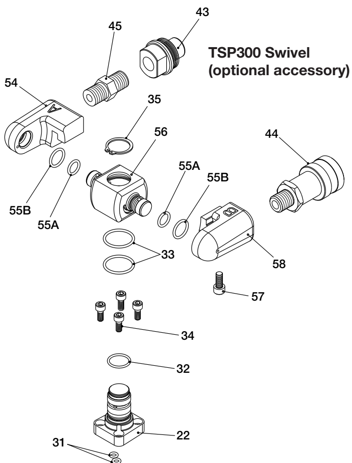
Figure 2, Swivel Assemblies, Model S11000X
