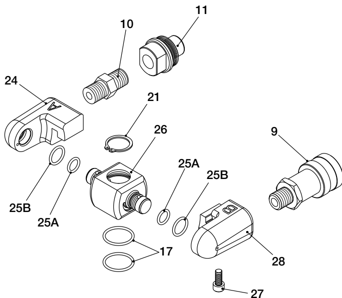
Figure 3, Drive Unit and Swivel Assemblies, W8000X Series
