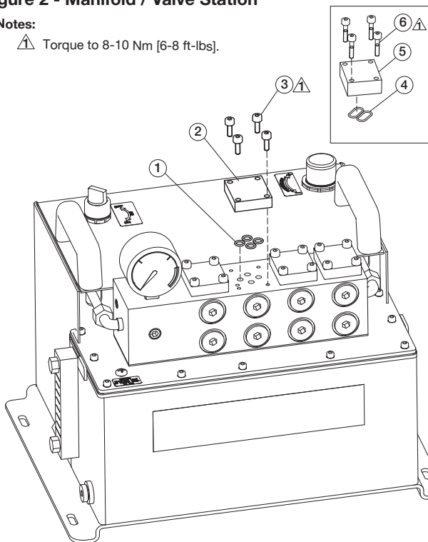
Figure 2 - Manifold / Valve Station
