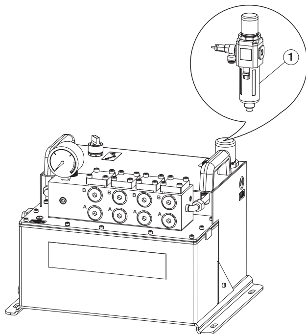
Figure 8 - Filter / Regulator
