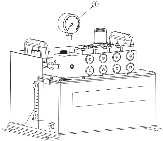
Figure 1 - Hydraulic Pressure Gauge
