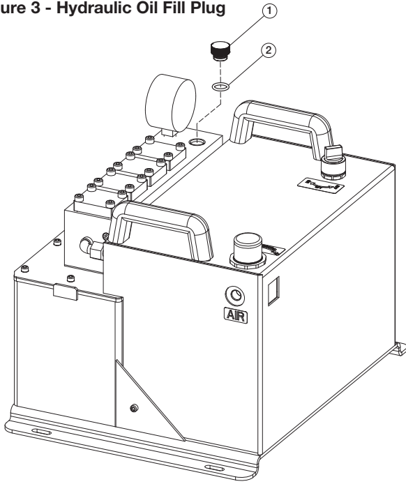
Figure 3 - Hydraulic Oil Fill Plug
