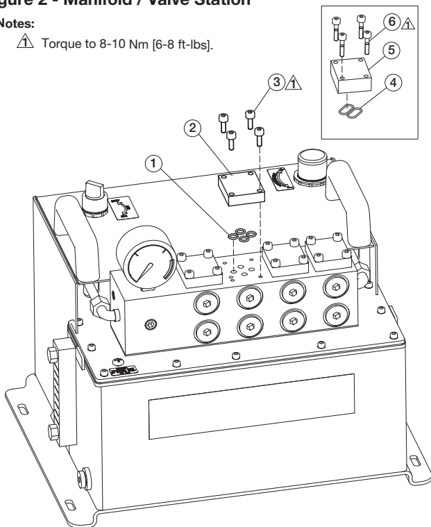
Figure 2 - Manifold / Valve Station
