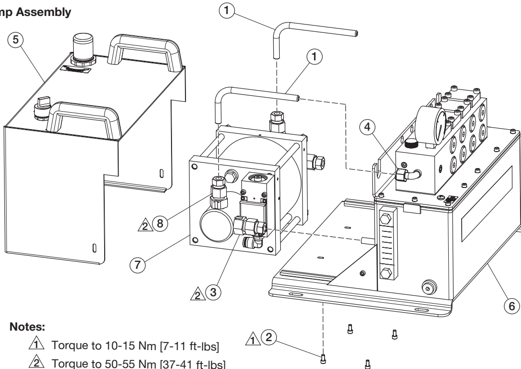
Parts List for Figure 4
