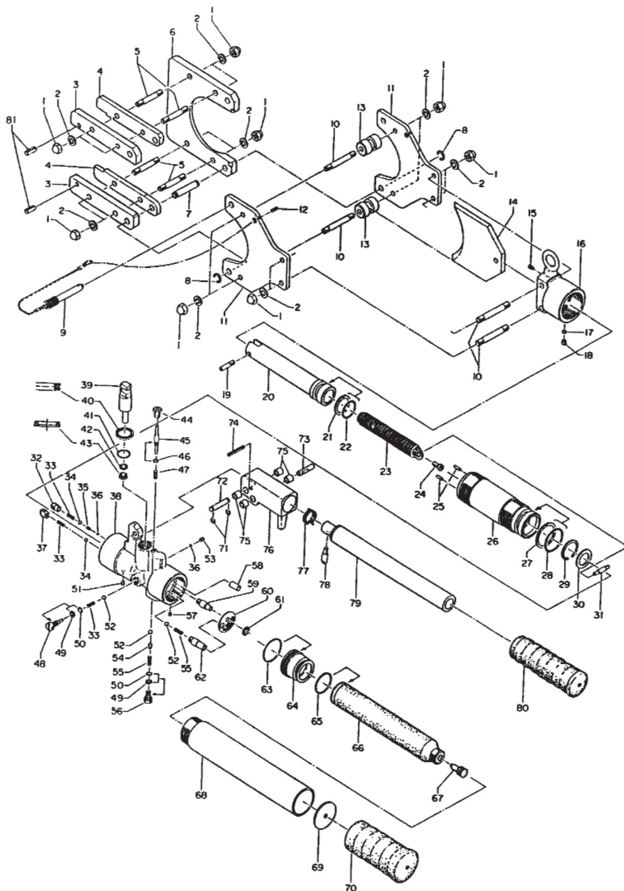
Figure 1: WMC3380 Hydraulic Cutter Exploded
