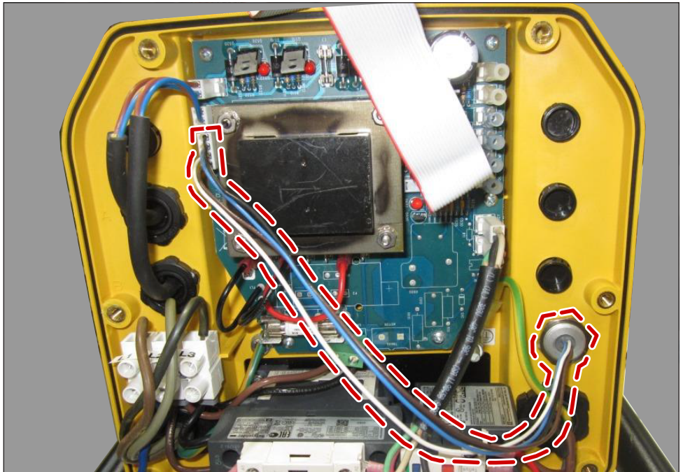
Figure 3 - Harness Assembly (electrical control box cover removed)
