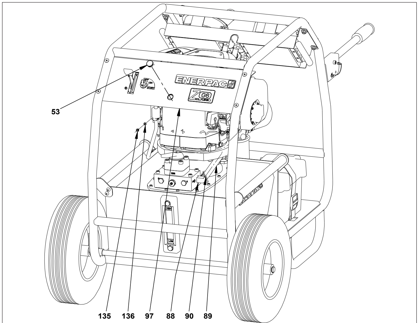
Figure 1, Main Assembly (2 of 2)
