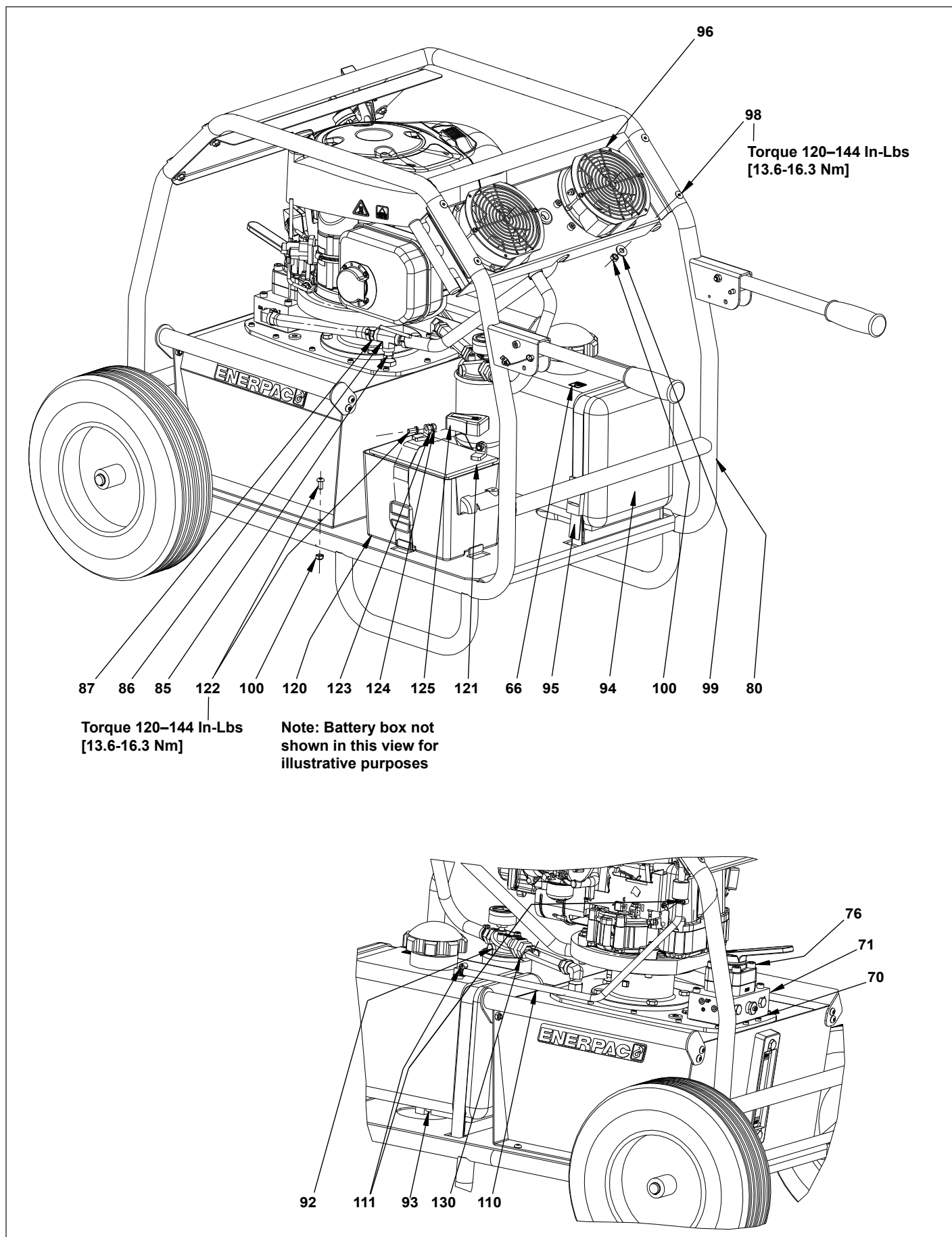
Figure 1, Main Assembly (1 of 2)
