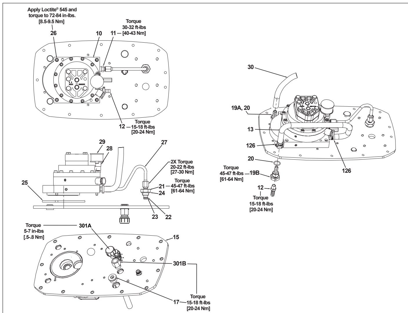
Figure 3, Pump Assembly (basic)
