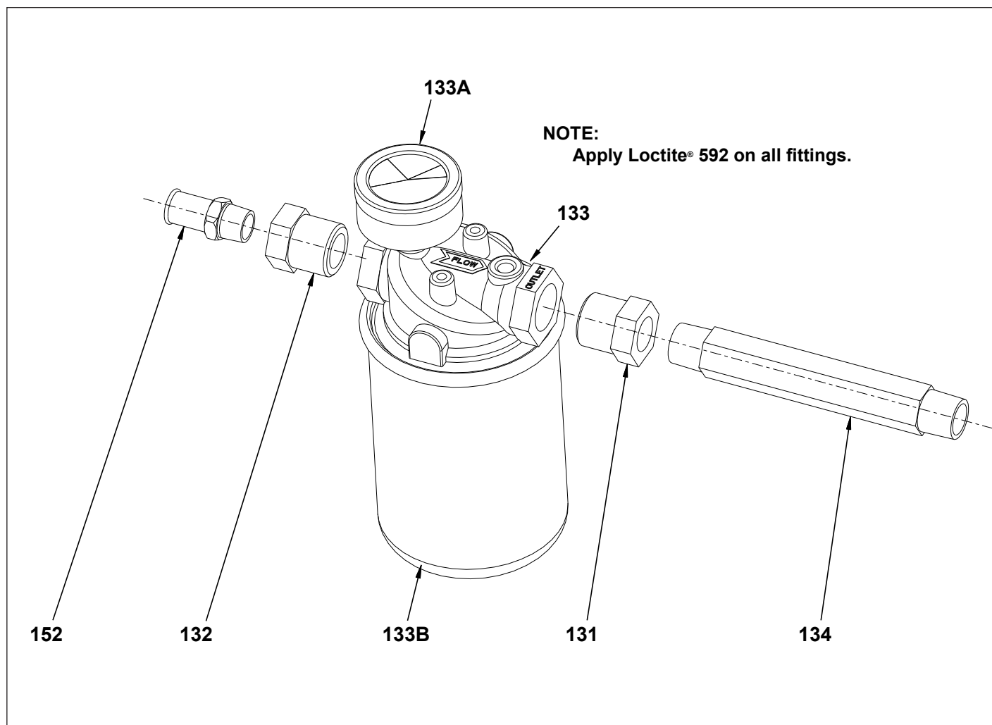
Figure 7, Oil Filter Assembly
