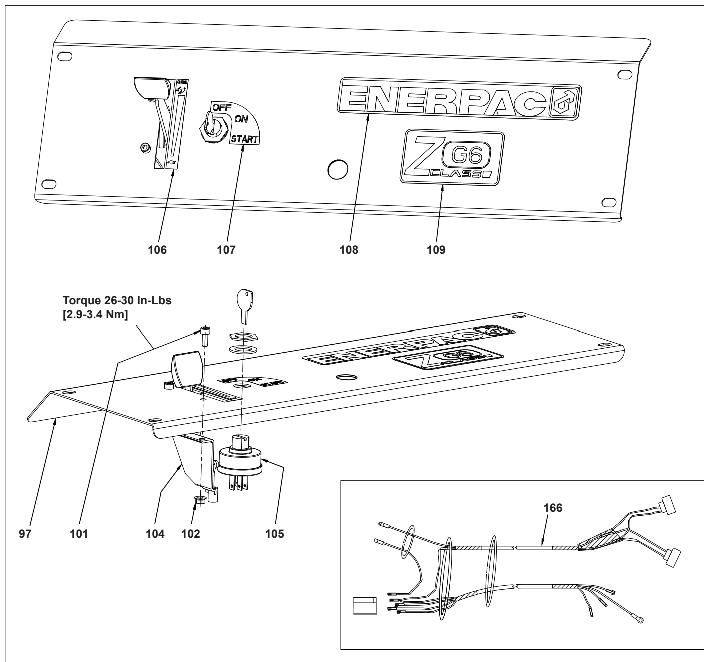
Figure 5, Control Panel Assembly
