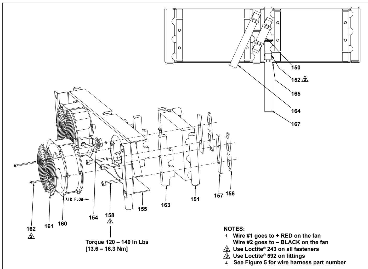
Figure 6, Heat Exchanger Assembly
