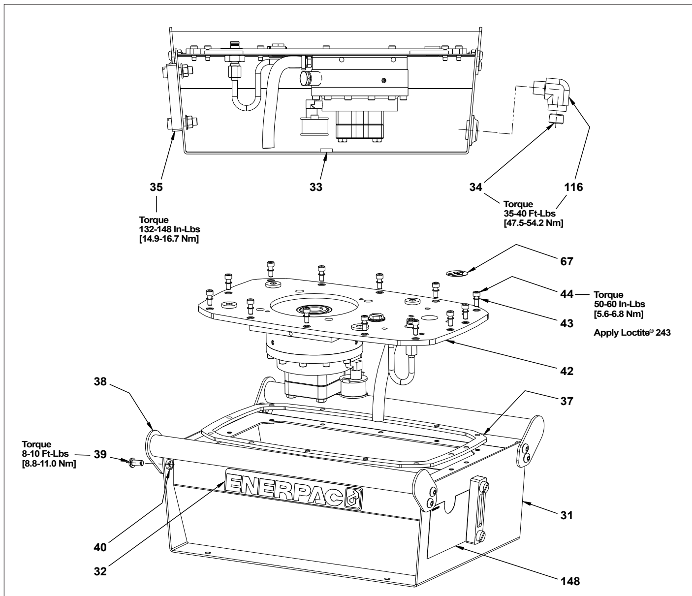
Figure 2, Pump and Reservoir Assembly
