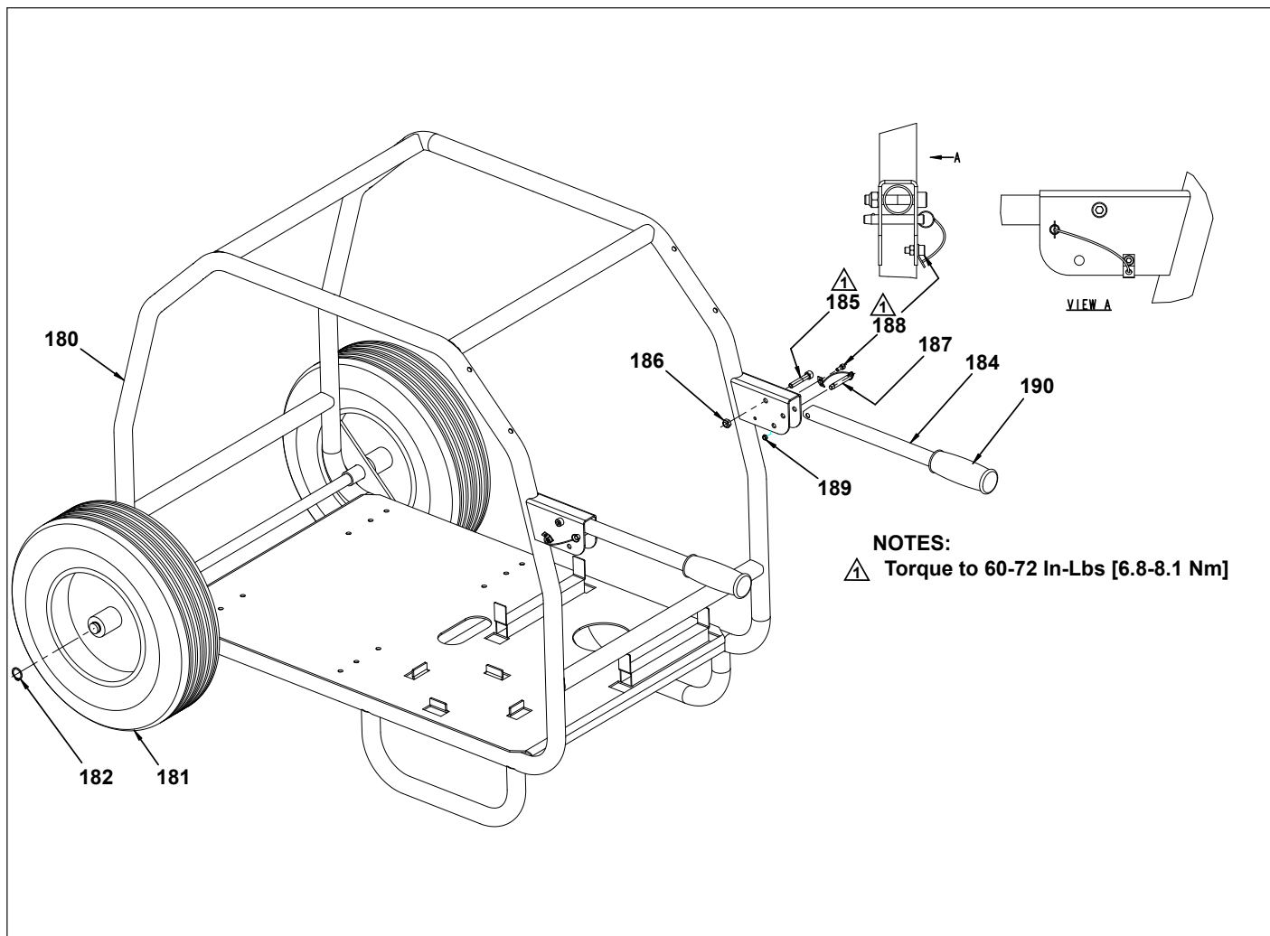
Figure 8, Cart Assembly
