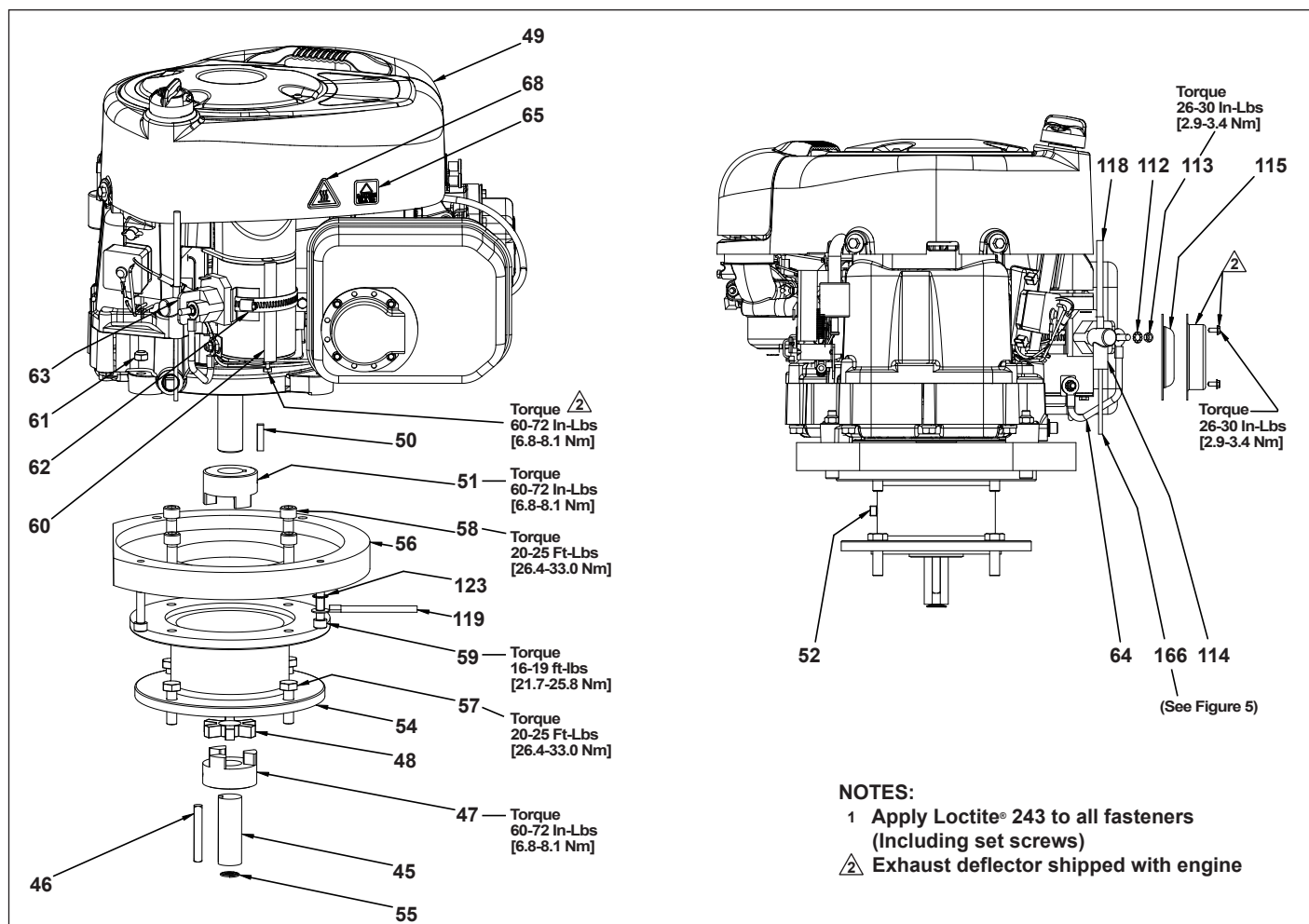
Figure 4, Engine Assembly (Briggs&Stratton)
