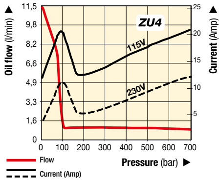
ZU4-SERIES PERFORMANCE CHART
