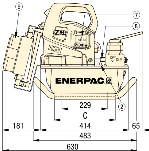
ZU4-Series with 4,6 and 6,8 litres reservoirs
