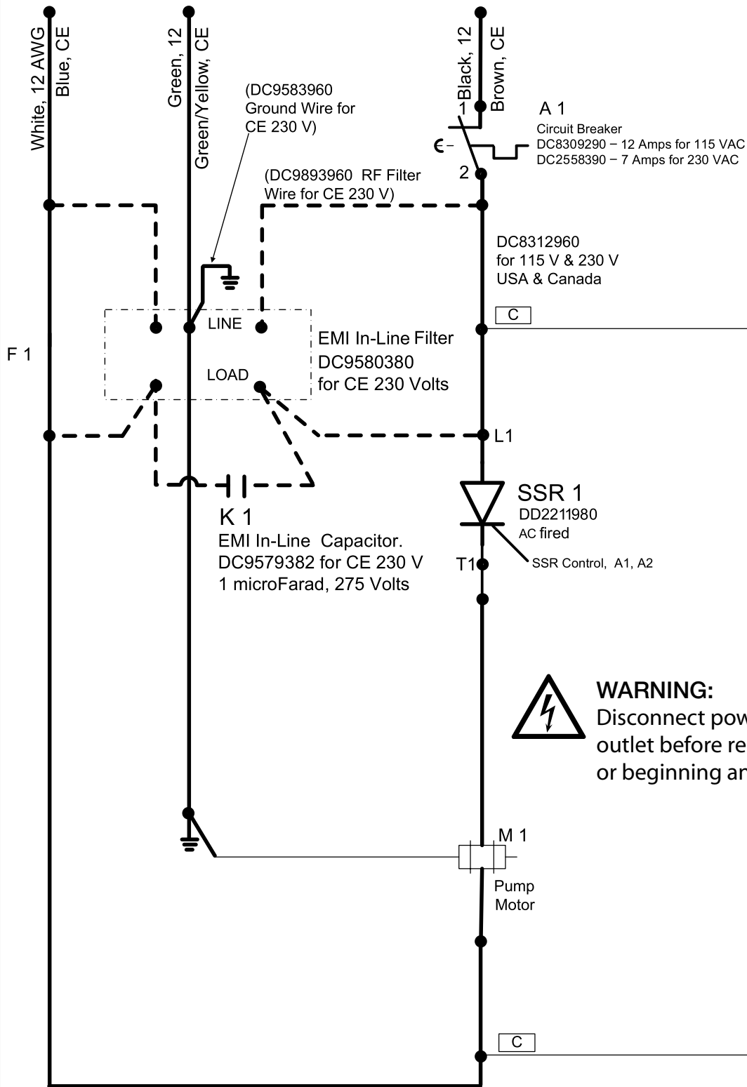
Figure 12, Electrical Diagram, ZUTP-1500 Electric Pump, Date Code "B" (View 1 of 2)
