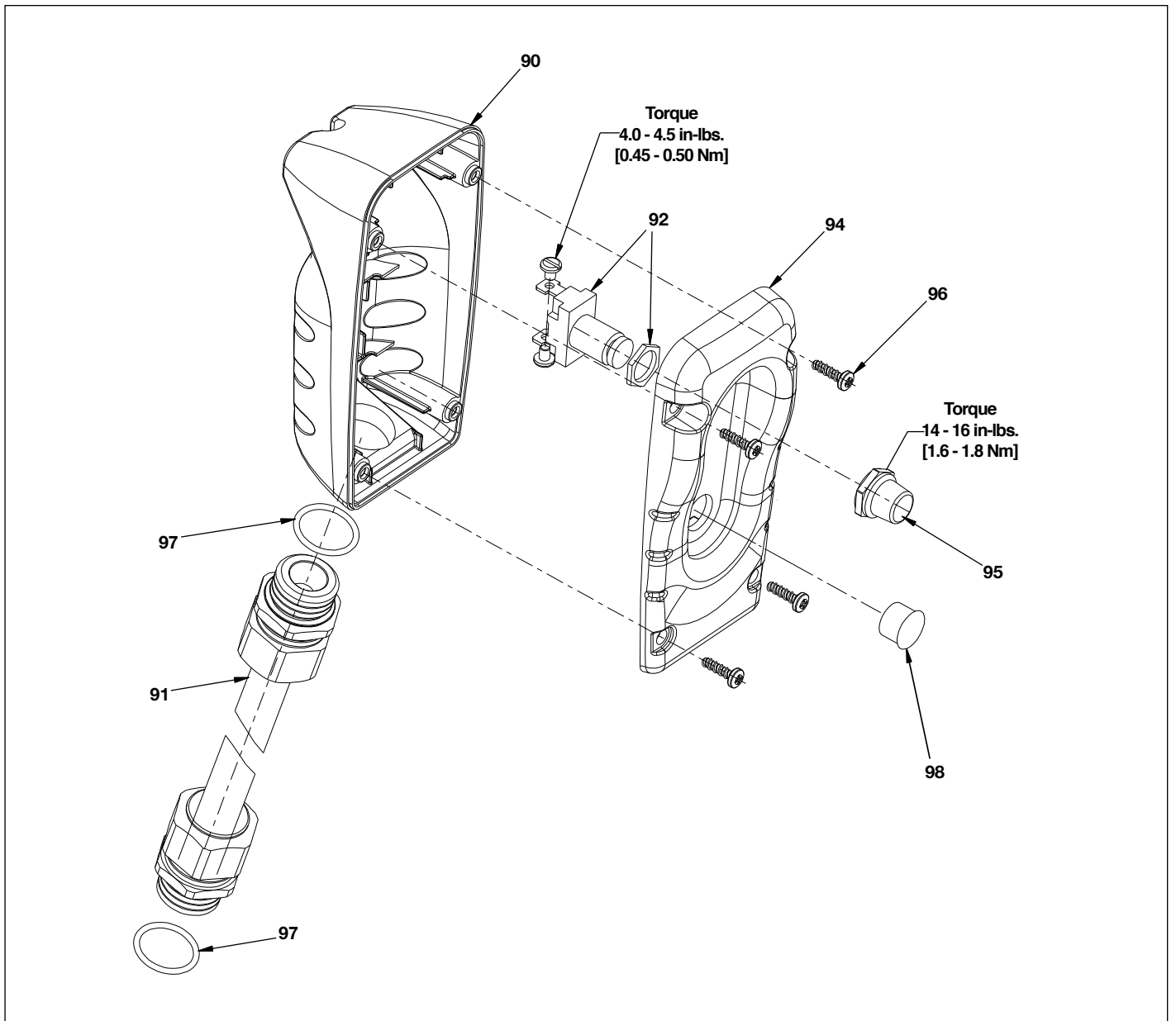
Figure 9, Pendant Assembly
