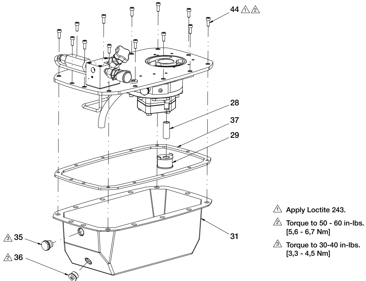
Figure 1, Reservoir and Coverplate Assembly
